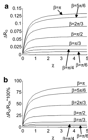
Figure 17. Difference in R_G between the intrinsically straight chain and the hinged chains with \Delta\beta = \pi/6 and different \beta . Part a presents the difference in absolute value, and part b presents the difference in percentage.
